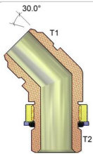
Jis Male To Bspp Male O-Ring 45° Adjustable Elbow Fittings
