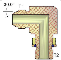
Male Komatsu To Metric Port Adjustable 90° Elbow
