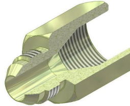
Male Jic To Female Komatsu 30 Deg. Cone
