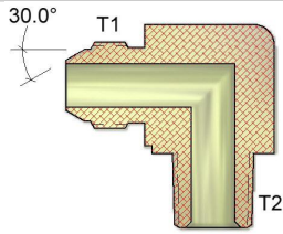
Male Komatsu To Male Bspt 90° Elbow
