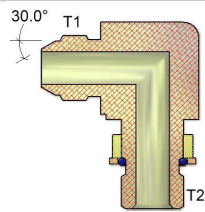
Male Komatsu To Bspp Male Adjustable 90° Elbow
