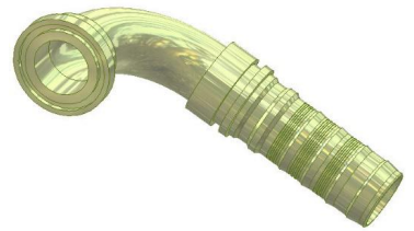
Flange Code 61 High Pressure 90°
