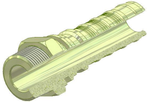
Male Bspt High Pressure
