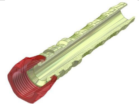
Female Jic Swivel High Pressure
