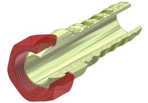
Female Bspp Swivel High Pressure
